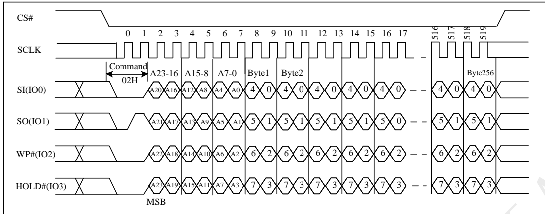
Figure 10-30a Page Program (PP) Sequence (QPI)
