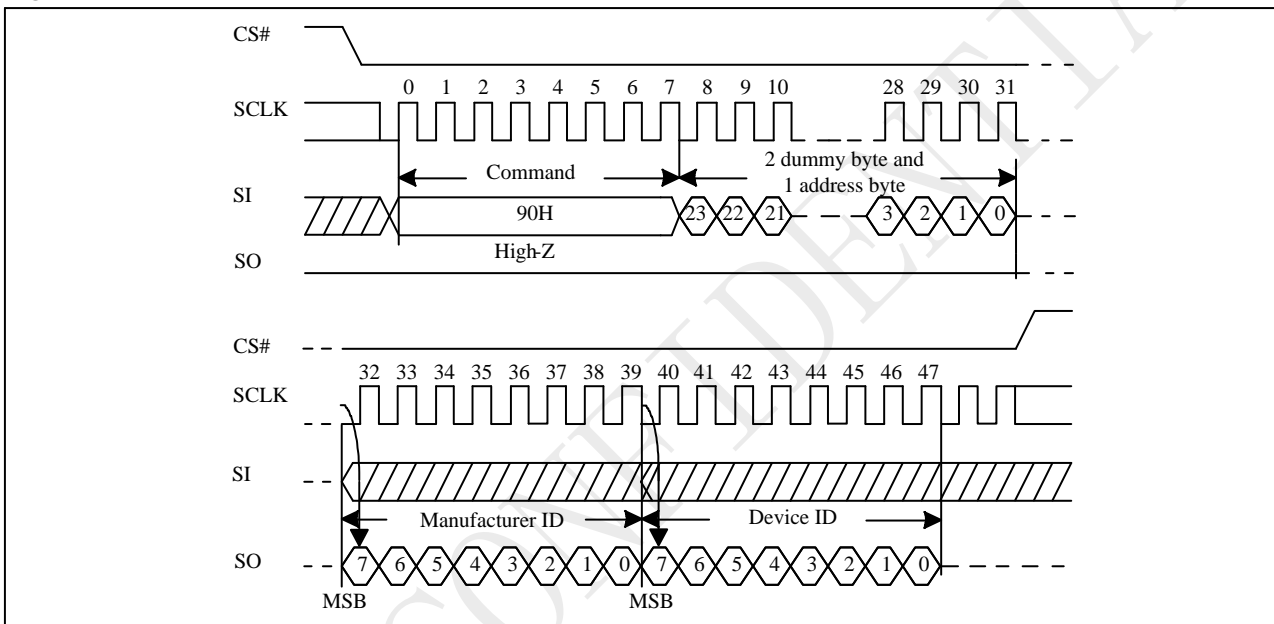
Figure 10-37 Read Electronic Manufacturer & Device ID (REMS) Sequence (Command 90h)
