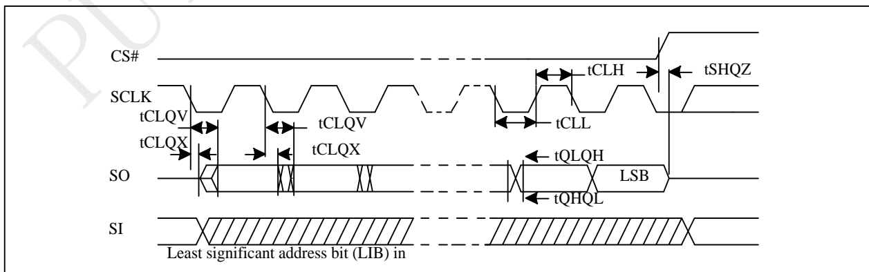
Figure 5-5 Output Timing
