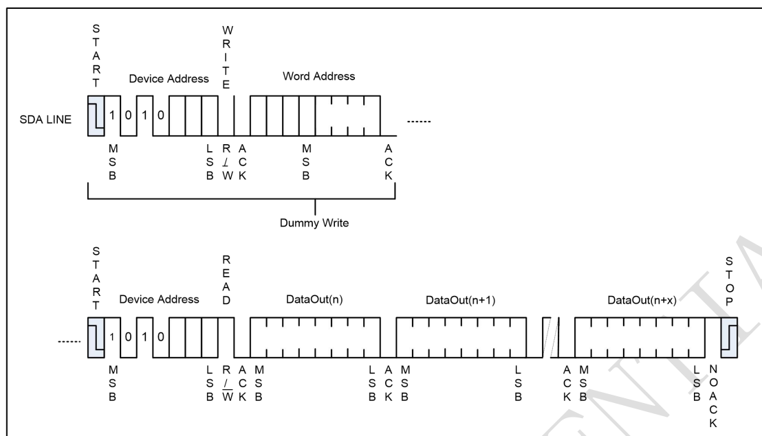
Figure 5-5 Sequential Read
