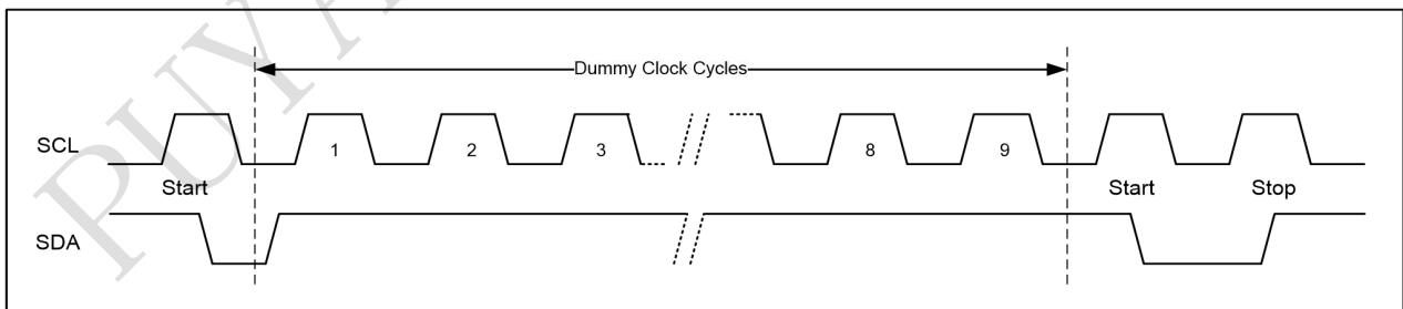
Figure 4-4 Soft Reset
