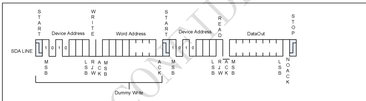
Figure 5-4 Random Read
