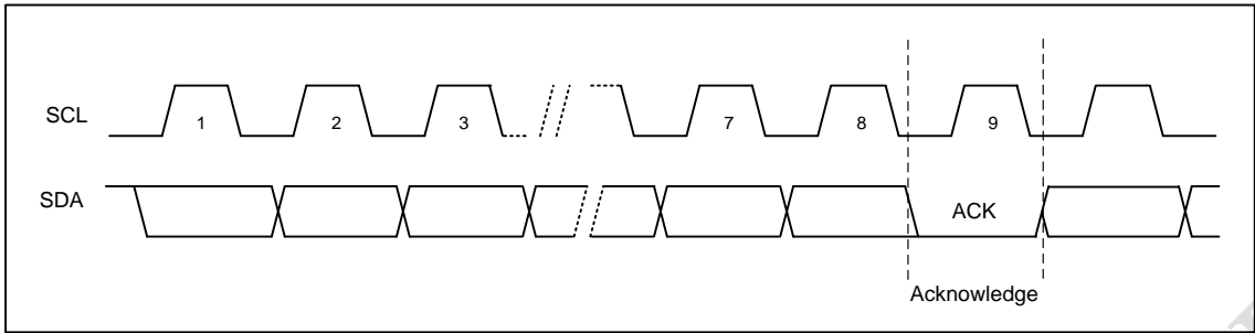
Figure 4-3 Output Acknowledge
