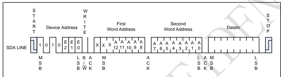
Figure 5-1 Byte Write
