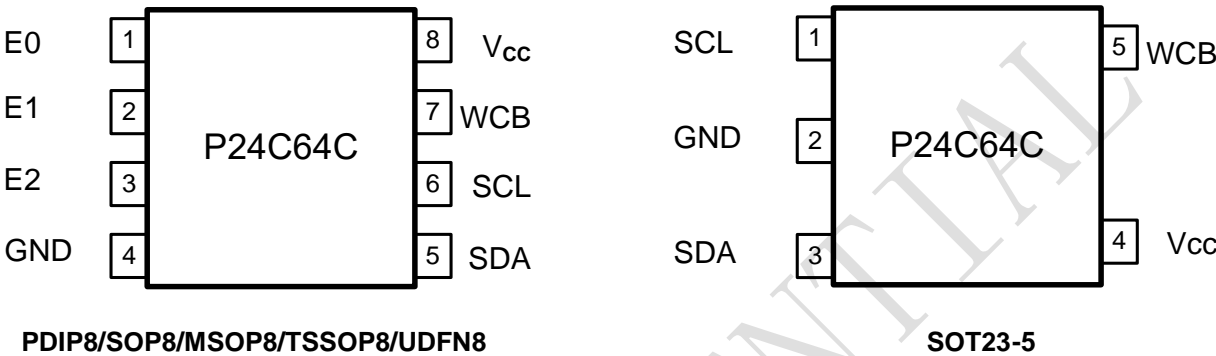
Figure 1-1 Pin Configuration
