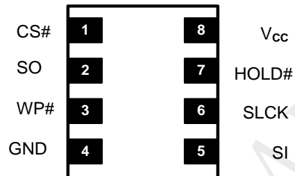
8-Land USON (2x3mm)
