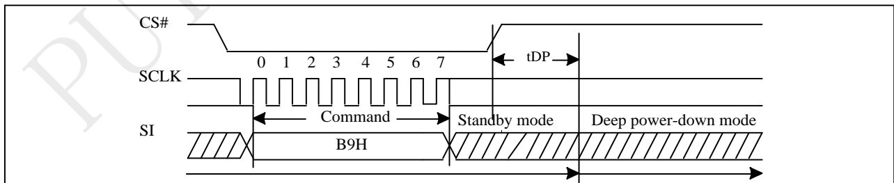
Figure 10-28 Deep Power-down (DP) Sequence (Command B9)
