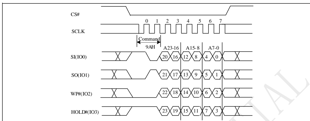
Figure 10-33a Buffer Load Sequence (QPI)
