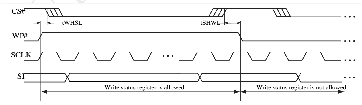
Figure 5-7 WP Timing
