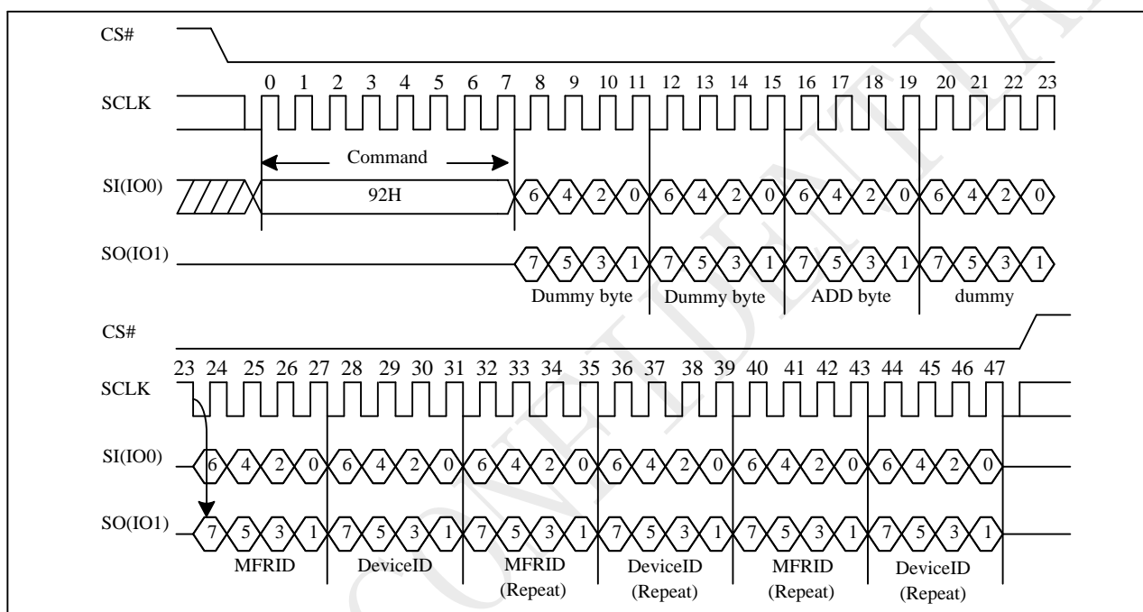
Figure 10-43 DUAL I/O Read Electronic Manufacturer & Device ID (DREMS) Sequence (Command 92)
