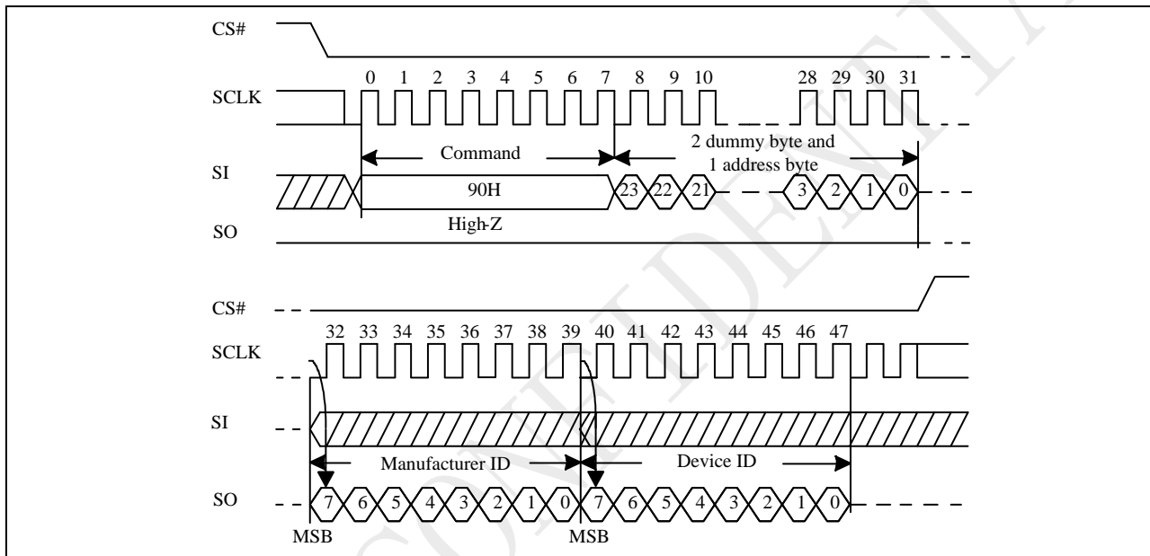
Figure 10-30 Read Electronic Manufacturer & Device ID (REMS) Sequence (Command 90)
