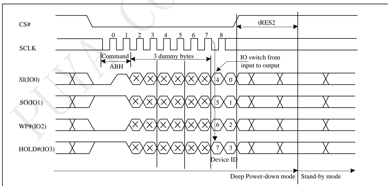
Figure 10-40a Read Electronic Signature (RES) Sequence (QPI)
