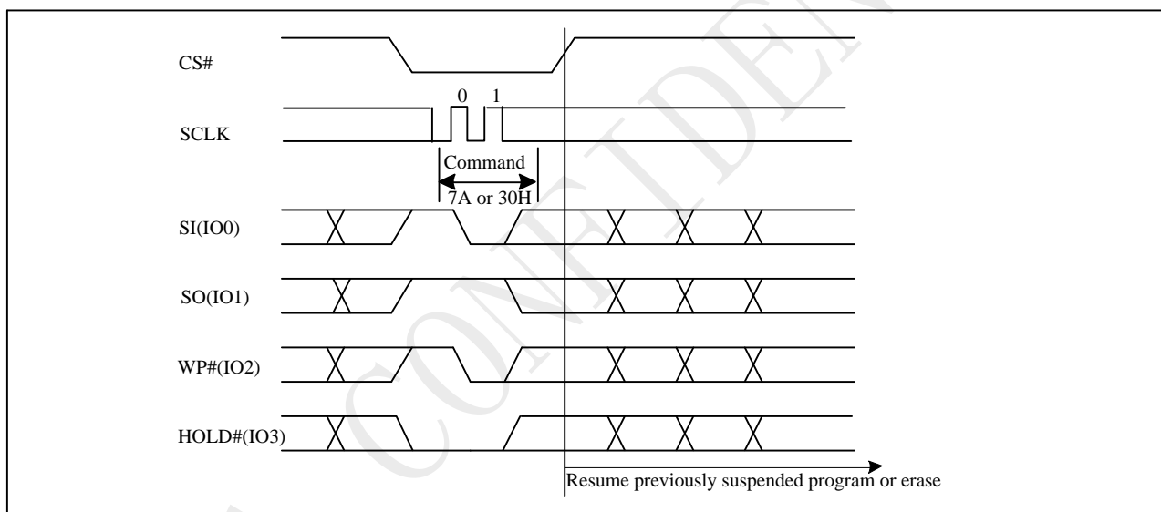
Figure 10-47a Resume to Read Latency(QPI)
