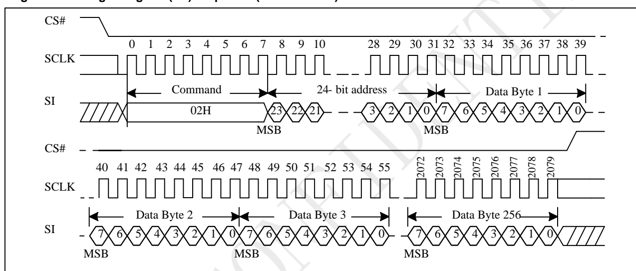
Figure 10-33 Page Program (PP) Sequence (Command 02)
