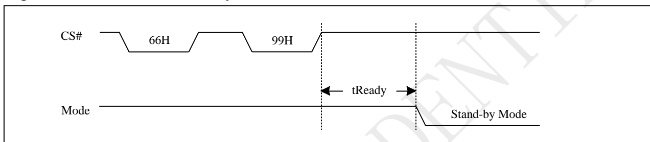
Figure 10-53a Reset Sequence
